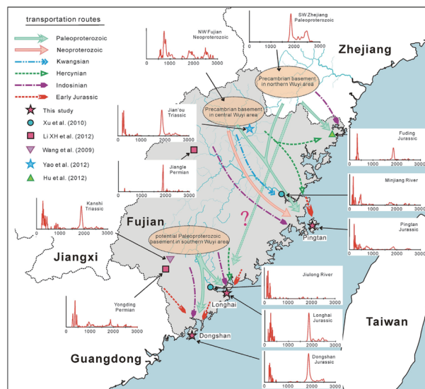
Fig. 10. Schematic diagram of the Wuyi terrane displaying the transport routes of terrigenous fragments in the Aojiao “Group” sediments. Data sources: Minjiang and Julong rivers (Xu and Chen, 2010); Fuding Jurassic (Hu et al., 2012); Kashi Triassic (Wang et al., 2009); Yongding and Jiangle Permian (Li XH et al., 2012); Jian’ou Triassic (Yao et al., 2012); NW Neoproterozoic (Wan et al., 2007); SW Zhejiang Paleoproterozoic (Yu et al., 2012).
