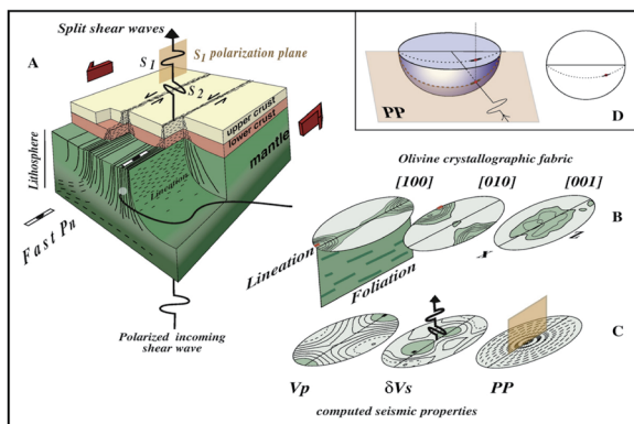
Fig. 12. Shear wave splitting in a transparent fault zone affecting the whole lithospheric mantle thickness (A). On this figure, a vertically incident polarized SWS wave propagates through a lithospheric mantle with a vertical foliation bearing a horizontal lineation. Transparent simple-shear causes the development of an olivine CPO (B) with [100] close to the lineation, [010] close to the normal to the foliation plane, and [001] orthogonal to the lineation in the foliation plane (orthorhombic symmetry). Panel (C) shows in the same structural referential the 3D seismic properties computed for this olivine CPO. The Vp diagram shows the highest P-wave velocity close to the maximum concentration of [100]-axis; the \delta V_s diagram shows the velocity difference between the fast and slow split S-waves for all propagation directions; the maximum birefringence is for S-waves propagating in a direction almost normal to the lineation, i.e. with a subvertical incidence in the case shown in (A). The PP diagram shows the orientation of the plane in which the fast S-wave is polarized; this plane is consistently defined by the fast S-wave propagation direction and the direction of the maximum concentration of [100]-axis (lineation). Panel (D) shows how the polarization plane is represented in a stereographic projection; to maintain visibility only a small segment of the intersection between the polarization plane and the lower hemisphere projected on the equatorial plane is shown.
