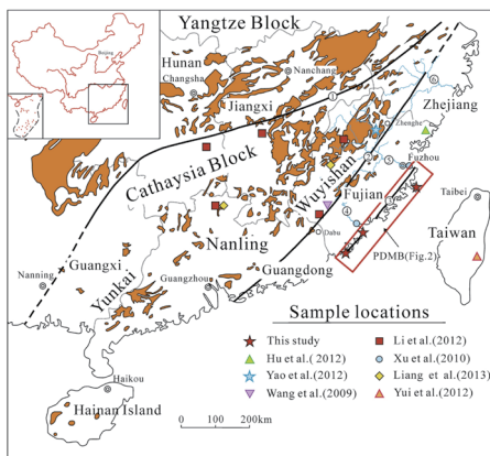
Fig. 1. Distribution of Precambrian rocks in the Cathaysia Block and sampling locations of Permian to Cretaceous sedimentary rocks in SE China. ① Jiangshan–Shaohing–Yuhuan–Pingtang Fault, ② Zhenghe–Dahu Fault, ③ Changle–Nan’ao Fault, ④ Julong River, ⑤ Minjiang River, ⑥ Oujang River.
